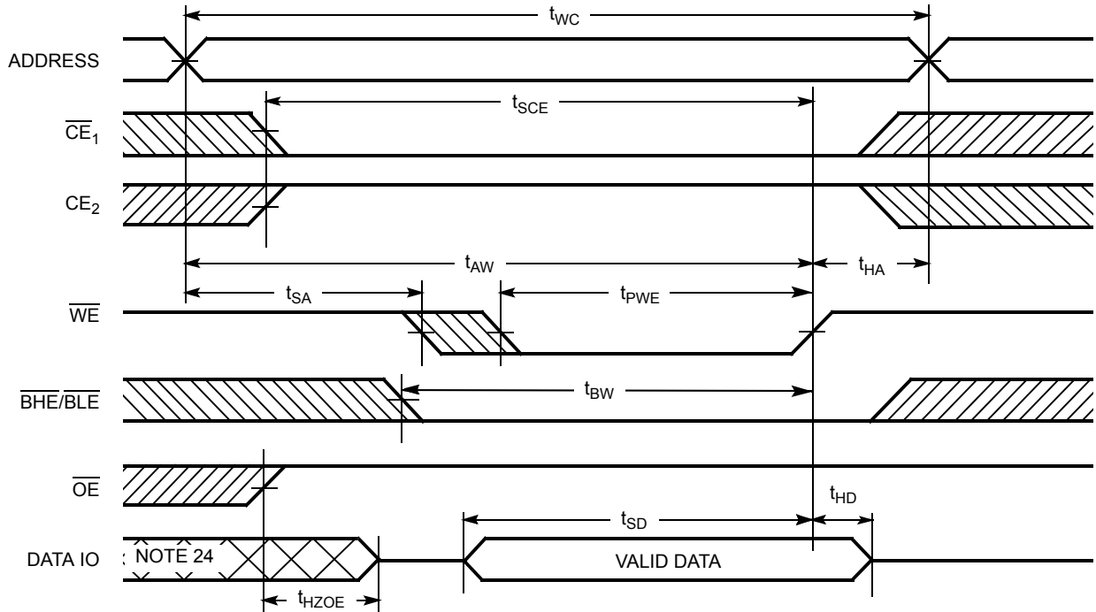
Write Cycle No. 2 ( \overline{CE}_1 or CE_2 Controlled) [18, 22, 23]
